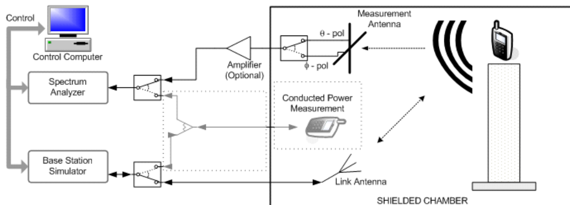
FIGURE A-25 SIMPLIFIED BLOCK DIAGRAM SHOWING A COMMON CONFIGURATION FOR THE USE OF A SPECTRUM ANALYZER POWER METER OR OTHER DEDICATED RECEIVER FOR TRP MEASUREMENTS. BOTH FORWARD AND REVERSE LINK COMMUNICATIONS BETWEEN THE MOBILE AND BASE STATION SIMULATOR ARE CARRIED OUT THROUGH A SEPARATE COMMUNICATION LINK ANTENNA.
