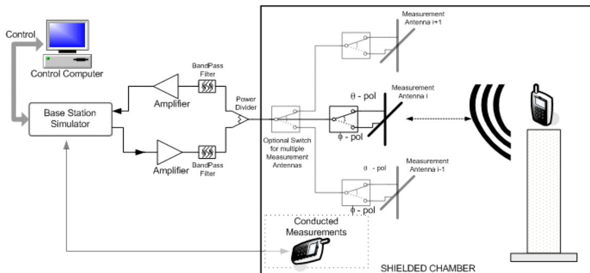
FIGURE A-27 SIMPLIFIED BLOCK DIAGRAM ILLUSTRATING A METHOD OF EXTERNALLY AMPLIFYING BOTH FORWARD AND REVERSE LINK COMMUNICATION SIGNALS AND COMBINING THEM INTO ONE SIGNAL ROUTED TO/FROM ONE (OR MORE) MEASUREMENT ANTENNA(S). THIS CONFIGURATION SUPPORTS BOTH TRP AND TIS MEASUREMENTS
